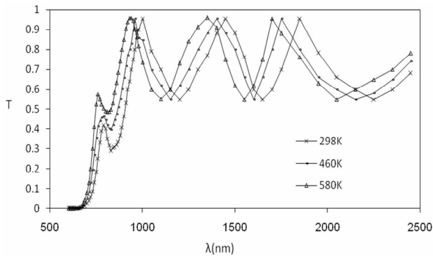
Fig.(3): Transmission spectra of \text{CdIn}_2\text{Se}_4 thin films (450 nm) as a function of wavelength at different substrate temperatures (298 K, 460 K and 580 K as representative example).
