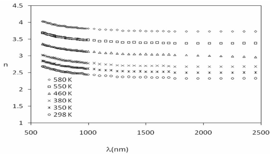
Fig.(6): Plot of refractive index, n versus \lambda for \text{CdIn}_2\text{Se}_4 thin films with different substrate temperatures
