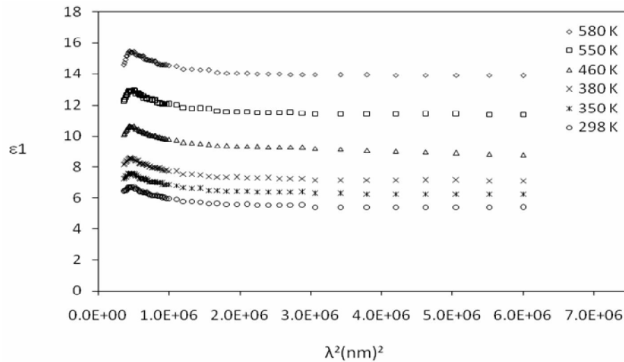
Fig.(7): Plot of \epsilon_1 versus \lambda^2 for \text{CdIn}_2\text{Se}_4 thin films deposited at different substrate temperatures.
