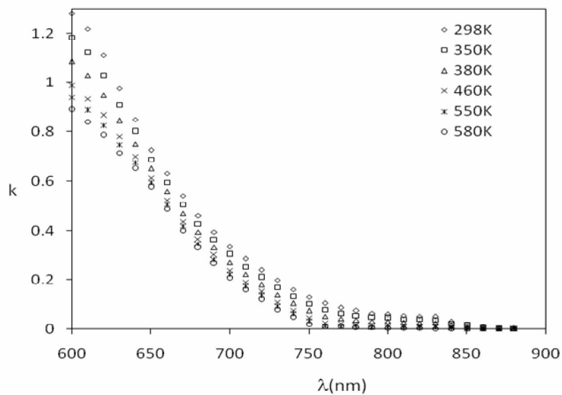
Fig.(4): The mean values of absorption spectra of \text{CdIn}_2\text{Se}_4 thin films with different substrate temperature
