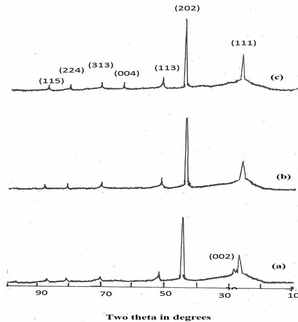
Fig.(1): XRD patterns of CdIn_2Se_4 films with thickness 450 nm at a) 298 K , b) 460 K and c) 580 K.
